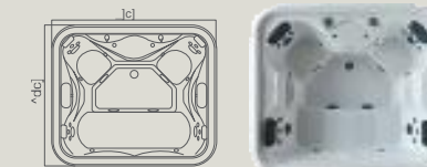
S-D-94 2060X1760X850
