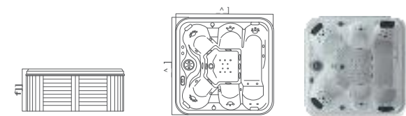
S-D-93A 2350X2000X900mm
